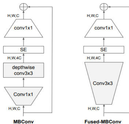
Fig.2. Structure of MBConv and Fused-MBConv [21]
