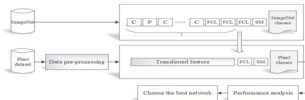
Fig.1. Illustration of the presented workflow diagram
